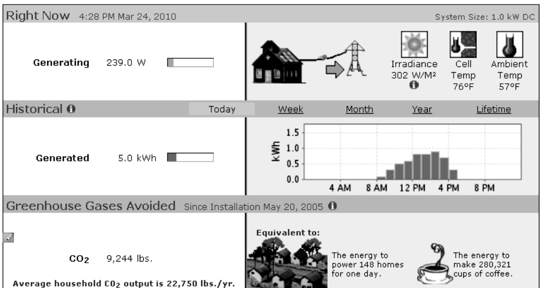
Figure 19.26 Monitoring display for 1 \text{kW}_p system [49]
