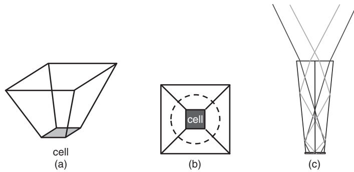
Figure 10.15 The most usual secondary optical devices. They are used to increase the limited gain of real Fresnel lenses (Courtesy UPM-IES)
