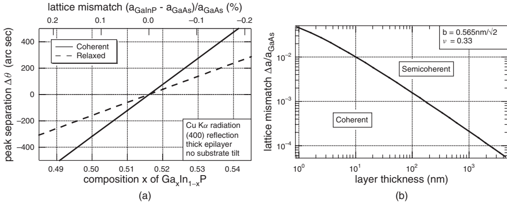
Figure 8.15 (a) A plot of \Delta\theta versus x for \text{Ga}_x\text{In}_{1-x}\text{P} on \text{GaAs} ; (b) plot of equilibrium boundary between coherent and semi-coherent epitaxy as a function of the absolute value of the epilayer lattice mismatch and thickness for a Poisson ratio \nu and a Burgers vector b , characteristic of \text{Ga}_x\text{In}_{1-x}\text{P}
