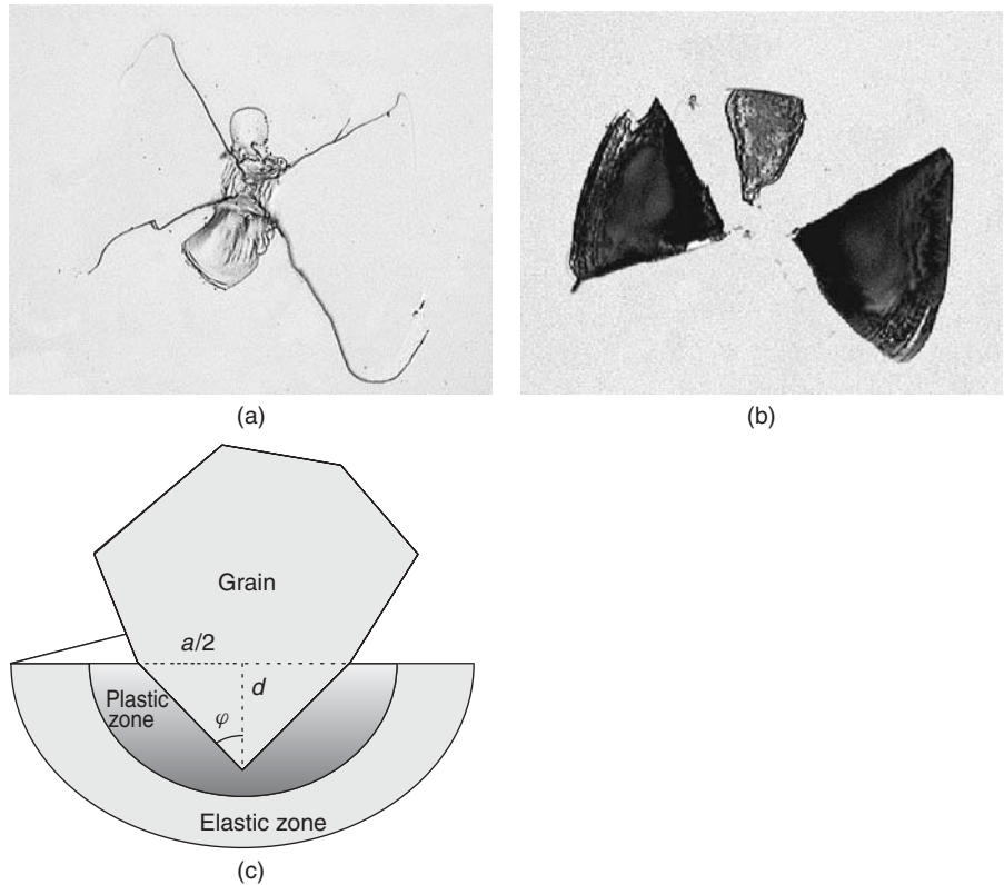
Figure 6.16 (a) Optical micrograph of median and (b) lateral cracks (below the surface) at a Vickers indentation. (c) Schematic representation of the impression of a sharp grain into a surface
