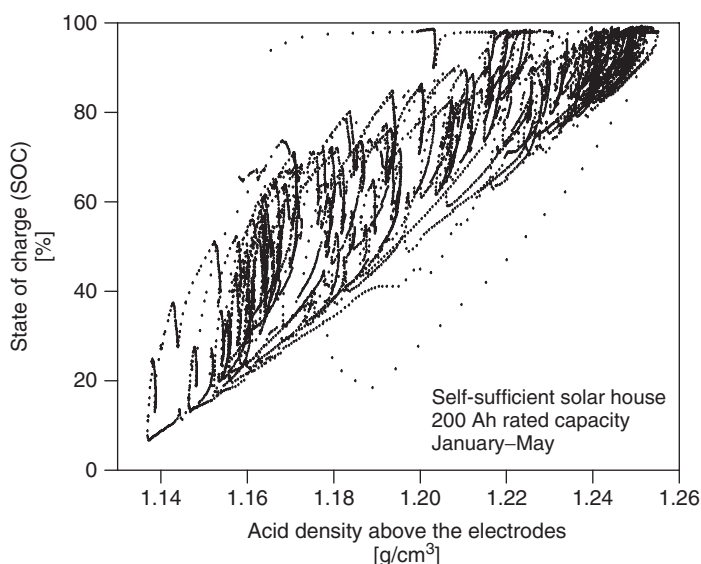
Figure 20.17 Acid density above the electrodes versus the actual state of charge, measured over five months for a battery from a photovoltaic system (200 A h cells, simulated acid densities based on measured initial data 10-minute average values)
