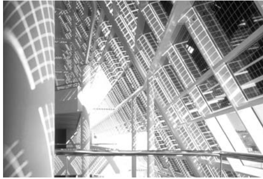
Figure 23.6 Solar office in Doxford Sunderland (UK) with a transparent double-glazing PV system integrated in the façade. The 73 kW p PV system is manufactured by Saint Gobain and mounted in Schüco window frames. Reproduced with permission by Dennis Gilbert
