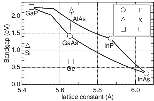
Figure 8.2 Estimated bandgap as a function of lattice constant for Si, Ge, and selected III-V binaries and their ternary alloys. The legend indicates the location of the bandgaps in the Brillouin zone; bandgaps located at the \Gamma point are direct
