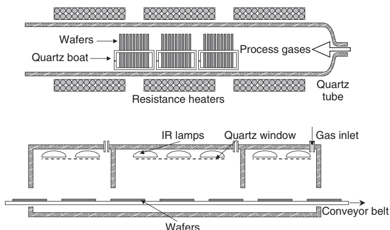
Figure 7.9 A quartz furnace (top) and a belt furnace (bottom) for the diffusion of phosphorus
