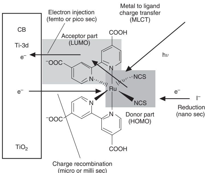
Figure 15.5 Schematic diagram of electron-transfer processes in DSSC. The dye is cis -dithiocyanato bis(4,4'-dicarboxy-2,2'-bipyridine)ruthenium(II) (N3 dye)
