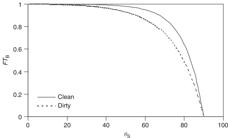
Figure 22.16 The relative transmittance FT_B is plotted against the angle of incidence \theta_S , for a clean surface and also for a dust-covered surface
