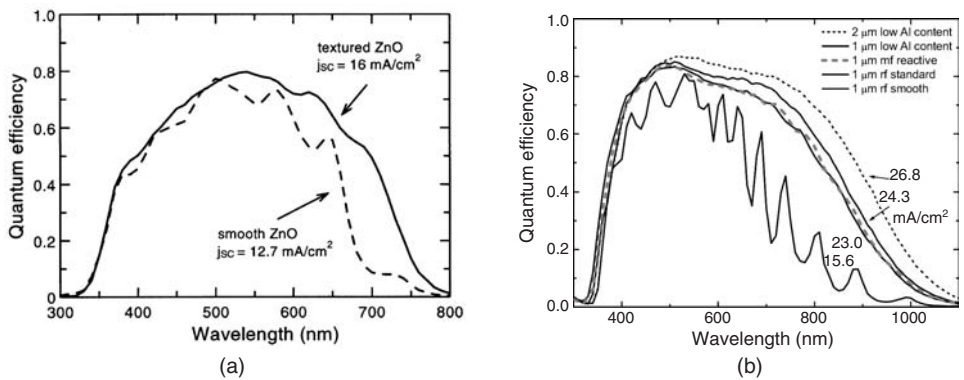
Figure 17.19 Quantum efficiency curves of (a) a-Si:H and (b) \mu c-Si:H p-i-n solar cells on smooth and texture-etched RF-sputtered ZnO:Al front contacts: (a) a-Si:H cell with 0.36 \mu m i -layer on ZnO:Al from 2 wt.% alumina ceramic ZnO target. Reproduced from Kluth O et al. , Thin Solid Films 351 , 247 (1999), with permission from Elsevier [223]; (b) \mu c-Si:H cell with i -layer thickness of 1.0 \mu m on ZnO:Al from standard (1 wt.%) and low (0.5 wt.%) alumina concentrations in the ceramic ZnO target, also on a surface-textured, reactive m.f.-sputtered ZnO film, and a \mu c-Si:H cell with i -layer thickness of 2.0 \mu m on low Al concentration ZnO. Reproduced from Rech B et al. , Thin Solid Films 511–512 , 548 (2006), with permission from Elsevier [256]
