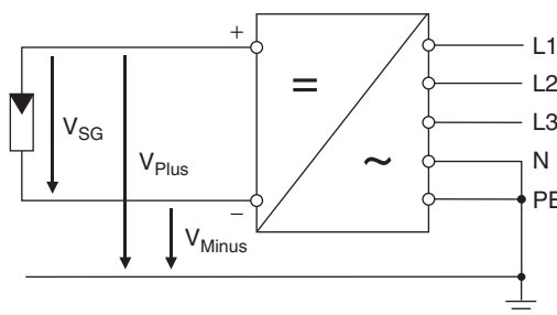
Figure 21.29 Definition of potentials at the input side of an inverter
