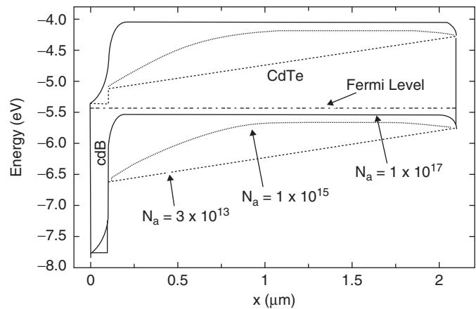
Figure 14.16 CdTe/CdS junction band diagrams at V = 0 for three values of CdTe acceptor density and a back-contact barrier
