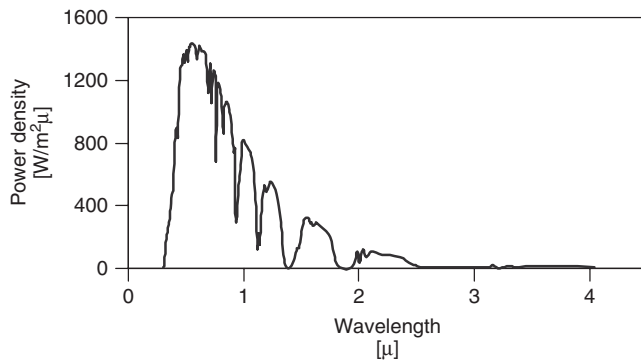
Figure 22.9 AM\ 1.5 solar spectrum, for an irradiance G = 1000 \text{ W/m}^2
