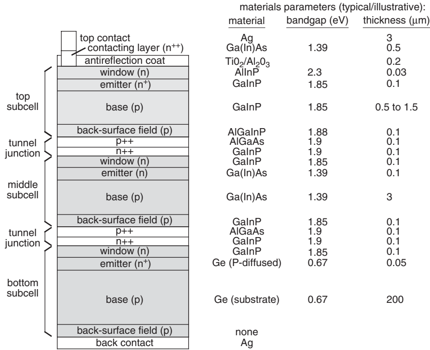
Figure 8.5 Schematic cross-section of a monolithic two-terminal series-connected three-junction solar cell. An n -on- p configuration is illustrated. Doping indicated by n^{++} , n^{+} , n (or p^{++} , p^{+} , p ) corresponds to electron (or hole) concentrations of the order of 10^{19} – 10^{20} , 10^{18} , 10^{17} respectively. Typical materials, bandgaps, and layer thicknesses for the realization of this device structure as a GaInP/GaAs/Ge cell are indicated. A back-surface field is not needed for the Ge junction because the base thickness is significantly greater than the minority-carrier diffusion length. Note that not all layers in an actual device (e.g. tunnel-junction cladding layers) are included in the illustration. The figure is not to scale
