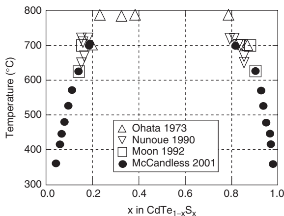
Figure 14.12 CdTe–CdS pseudobinary equilibrium phase diagram. (Data listed in order from References [160, 78, 161, 170])
