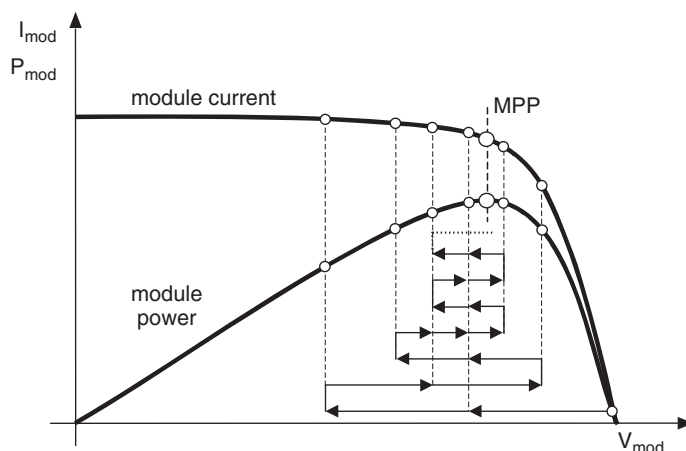
Figure 21.8 Working principle of the “mountain-climb” MPP-tracking algorithm
