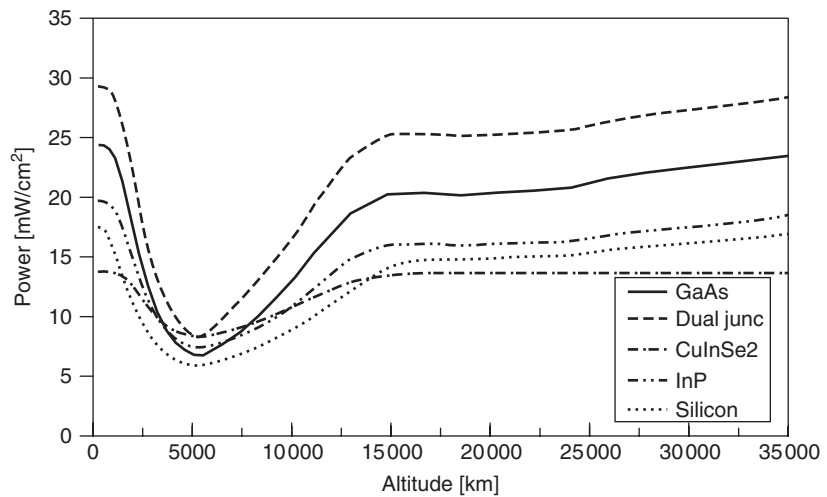
Figure 9.4 Solar cell power density as a function of altitude after 10 years in a 60° orbit with a coverglass thickness of 300 \mu\text{m} (GaAs: BOL 24.4 ( \text{mW/cm}^2 ) [37]; Dual Junc – GaInP/GaAs/Ge [38]: BOL 29.3 ( \text{mW/cm}^2 ); CuInSe2: BOL 14.4 ( \text{mW/cm}^2 ) [39]; InP: BOL 19.7 ( \text{mW/cm}^2 ) [40]; Si: BOL 17.5 ( \text{mW/cm}^2 ) [41]). (Graph courtesy of Tom Morton, Ohio Aerospace Institute)
