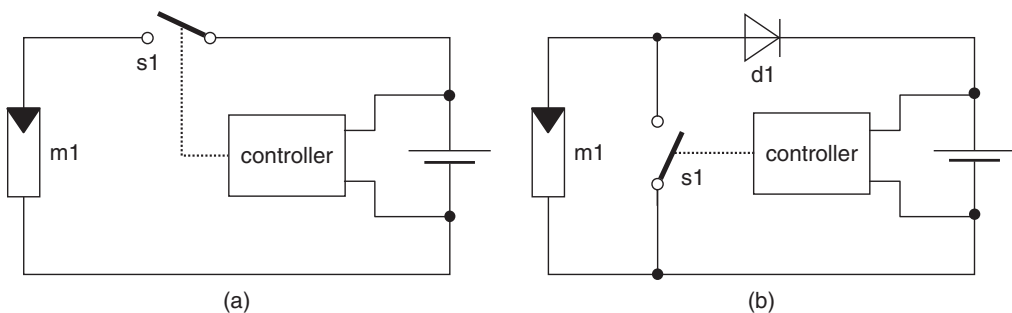
Figure 21.4 Principle of (a) series and (b) shunt switching controllers
