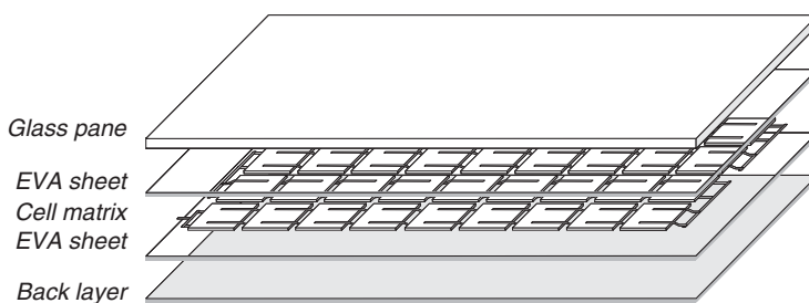
Figure 7.18 Stack of materials to be laminated
