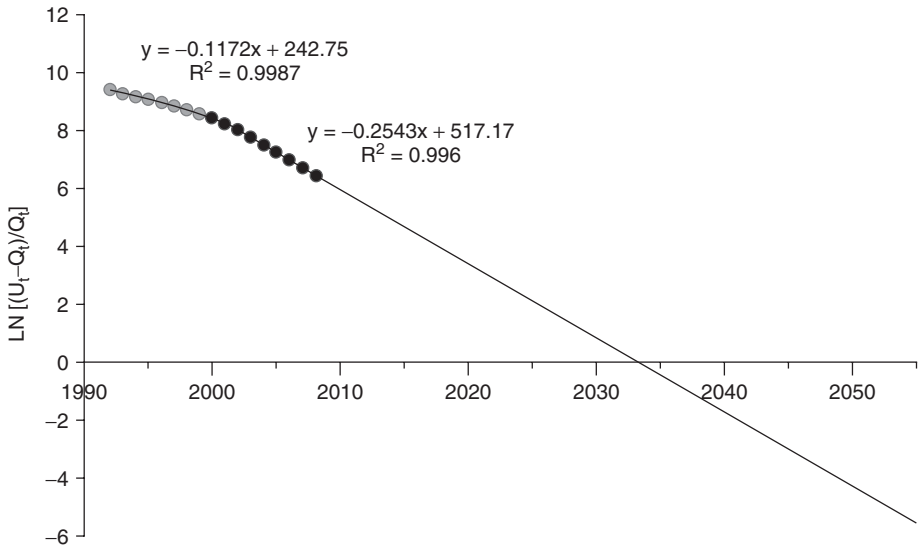
Figure 2.15 Regression analysis using a logistic growth model for US PV installation. Data sources: [12, 123]
