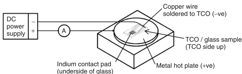
Figure 17.23 Set-up for TCO/glass delamination test showing indium contact to the glass and connections to the electrically-isolated DC power supply. Adapted from Jansen K, Delahoy A, Thin Solid Films 423/2 , 153 (2003) [281]
