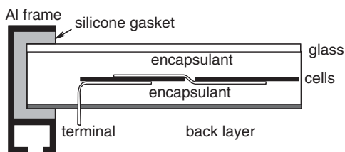
Figure 7.19 Cross- section of a standard module
